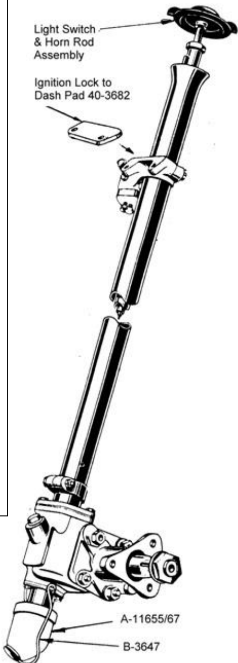
1933-34 Steering Column Assembly
