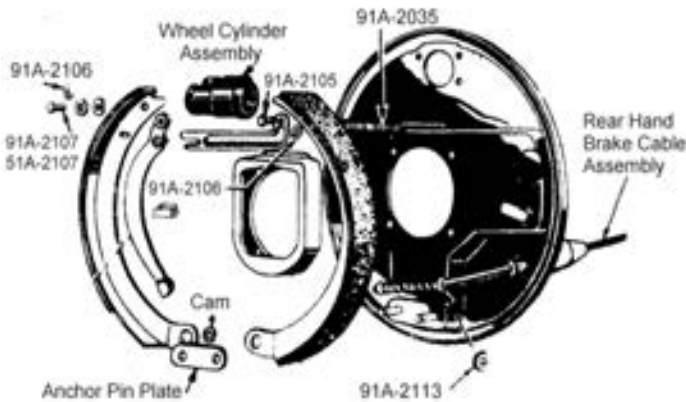
REAR BACKING PLATE COMPONENTS
