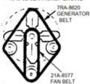
1949-52 8BA PICKUP ENGINE
