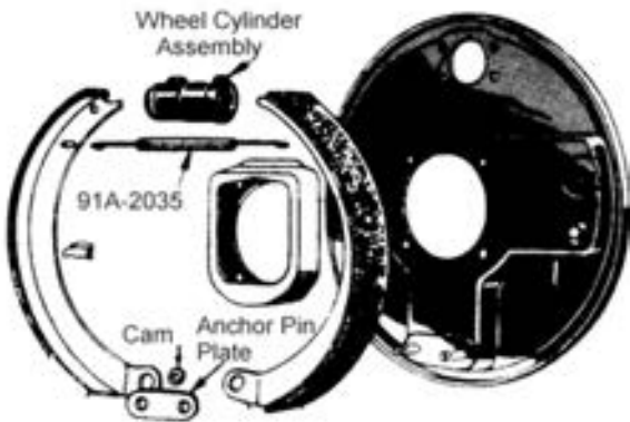
FRONT BACKING PLATE COMPONENTS
