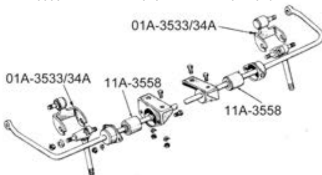
1940-41 Deluxe Sway Bar
