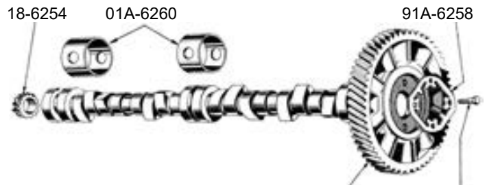
Camshaft Timing Gear 350400-S
