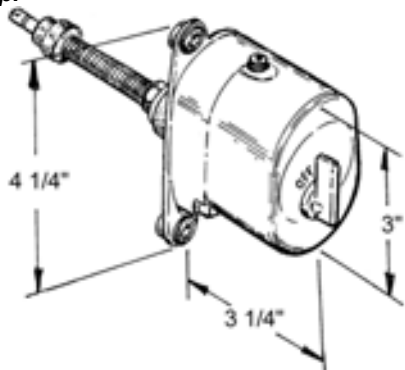
Dimensional for A-17508 electric motors listed above & below
