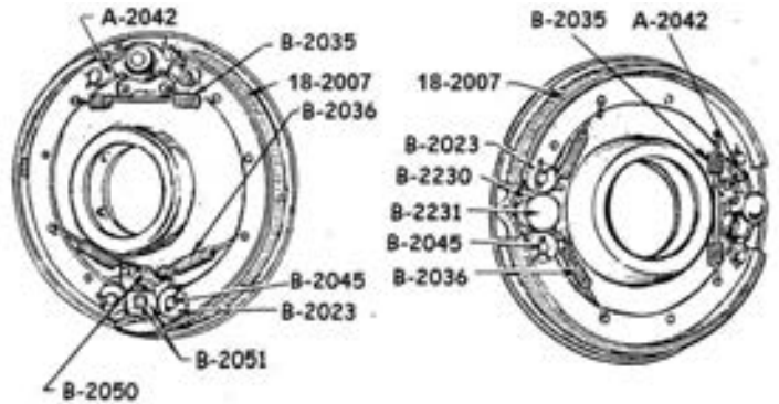
1933-1934 Brake System
