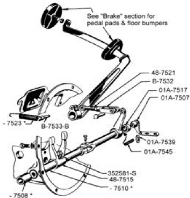
1940-48 Passenger Clutch Pedal & Parts
