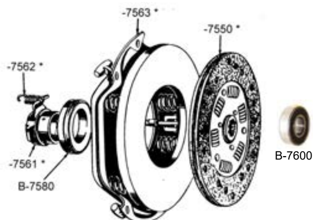
Typical Clutch & Pressure Plate Components
