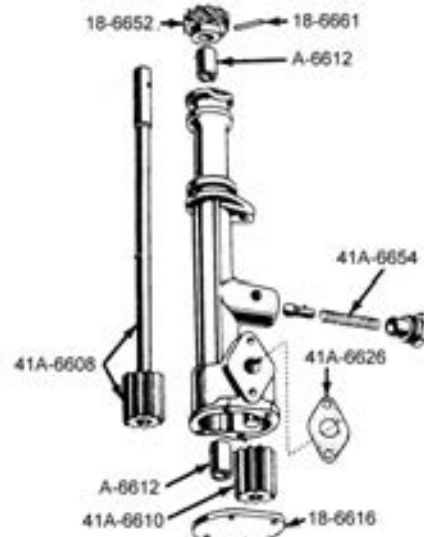
80# Pressure Oil Pump
