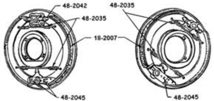
1935-1936 Brake System
