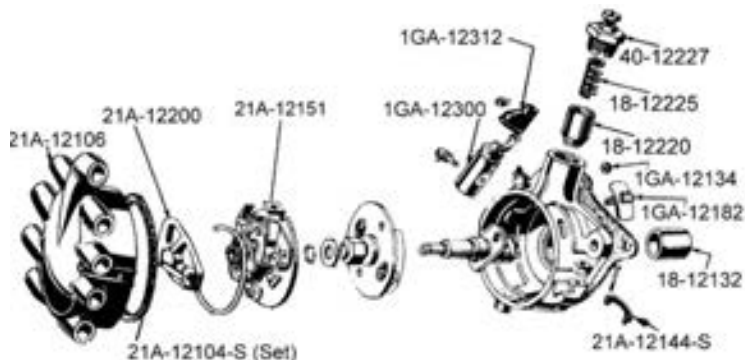
1942-44 V8 Distributor
