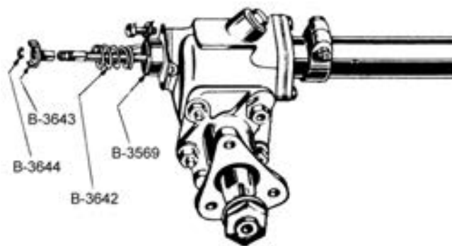
Typical Steering Box Assembly Detail (1933-34 Shown)
