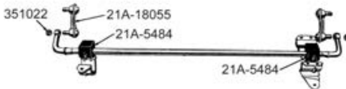
1942-48 Passenger Stabilizer
