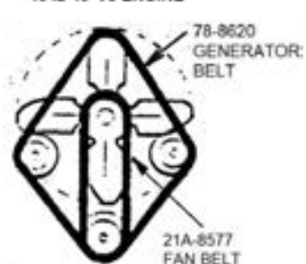
1942-48 V8 ENGINE
